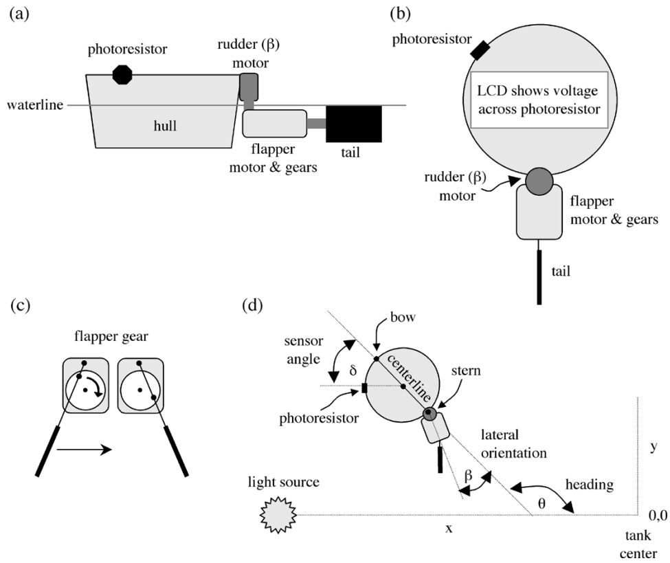
Fig. 2. Design of the autonomous surface-swimming robotic tadpole. (a) Side view. (b) Top view. (c) The flapper gear, showing extreme lateral positions of tail. (d) Coordinate system and definition of robot heading \theta , lateral orientation of tail \beta , and sensor angle \delta .
